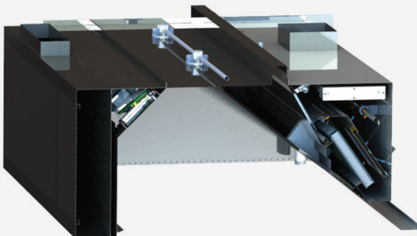
Kitchen hood Construction & Section Details
