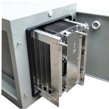
Dry Scrubber Cleaning Method
